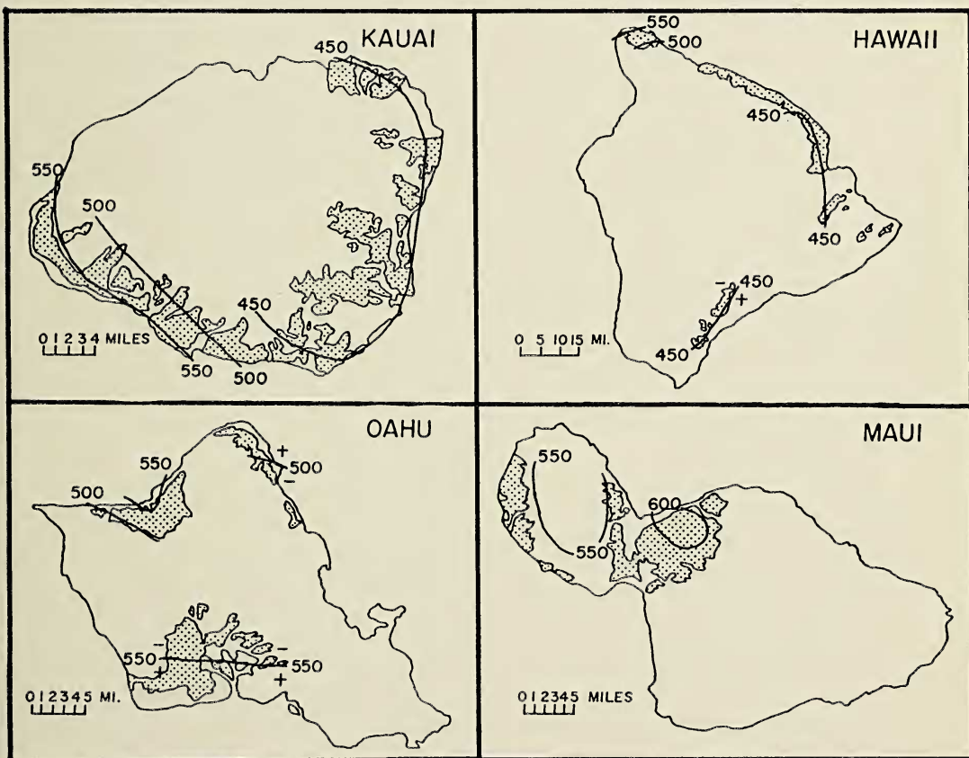
FIG. 8. Solar radiation (langley/day) in Hawaii.
